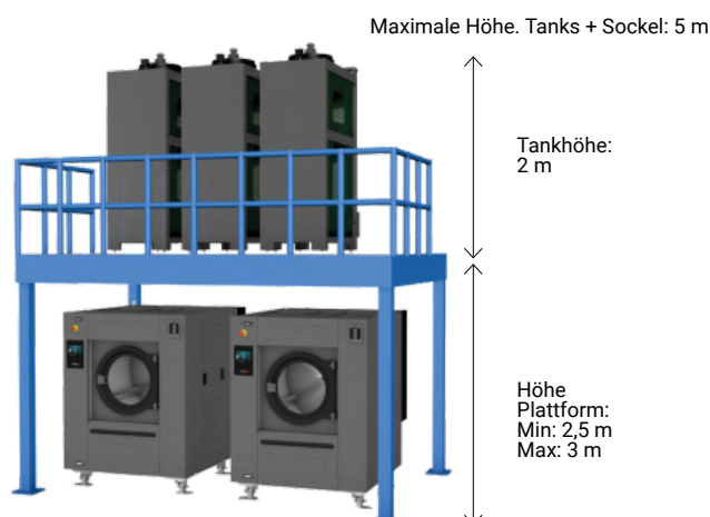
OPTION HOCHINSTALLATION
